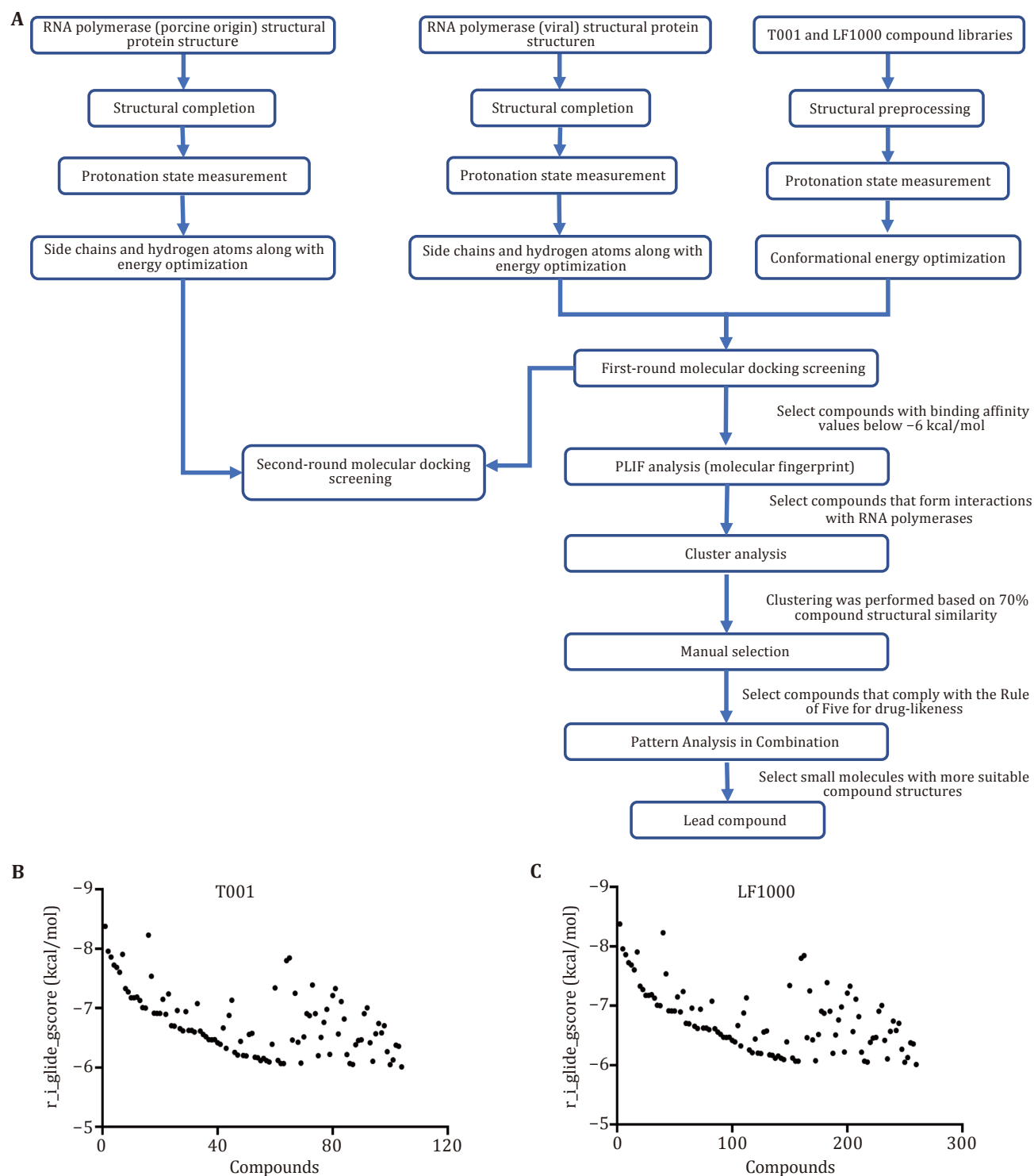
Fig. 2 Virtual screening workflow and docking score distributions. A Schematic of the virtual screening pipeline, including protein preparation, ligand processing, molecular docking, and selection criteria. B,C Docking score distributions for candidate compounds from the T001 ( B ) and LF1000 ( C ) libraries
