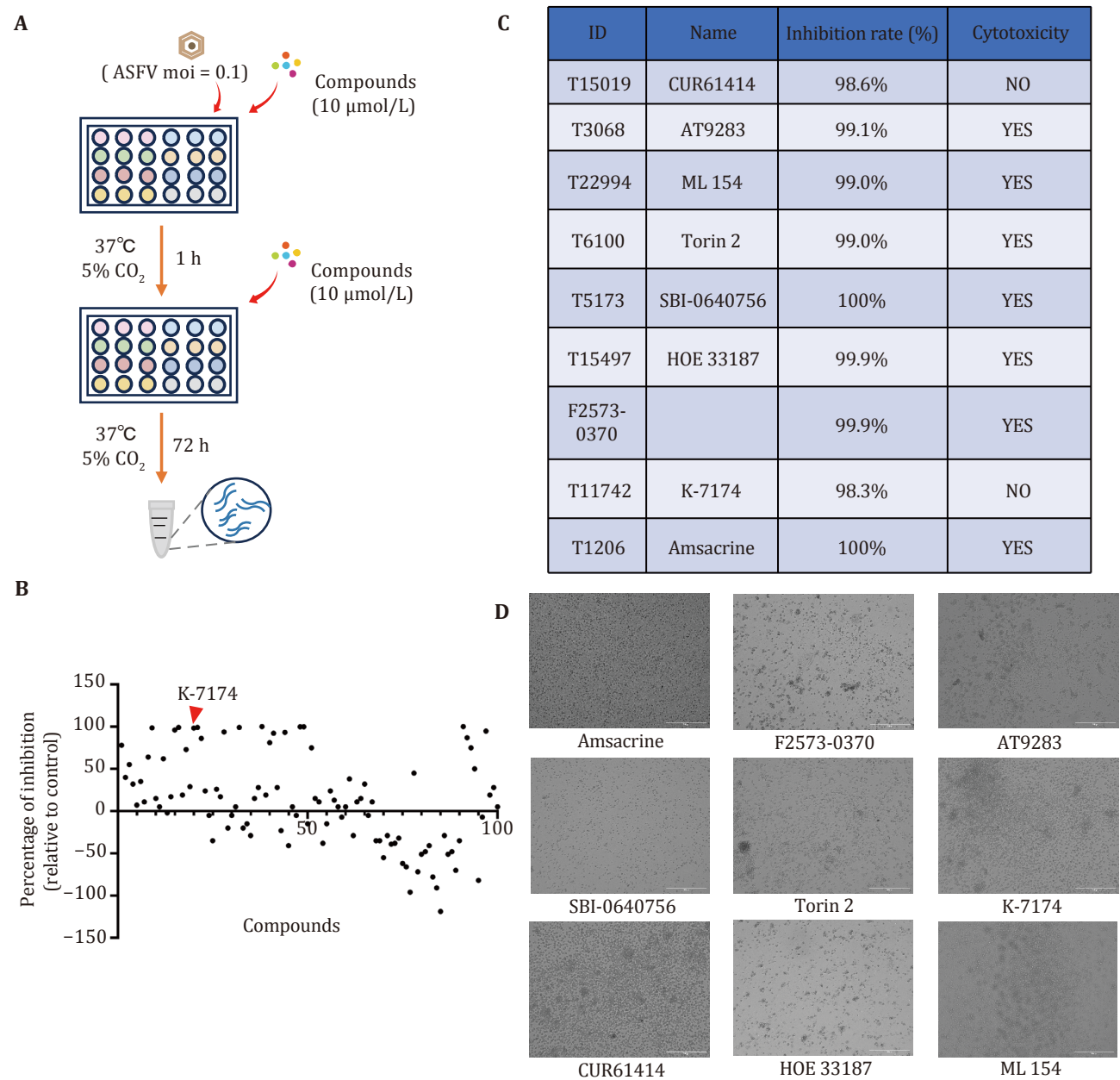
Fig. 3 In vitro screening of candidate compounds for anti-ASFV activity. A Experimental timeline for antiviral assessment in PAMs. B Inhibition rates of 100 candidate compounds at 10 \mu\text{mol/L} . C Inhibition rates and cytotoxicity profiles of the top nine hits. D Cell viability of PAMs treated with the top nine compounds
