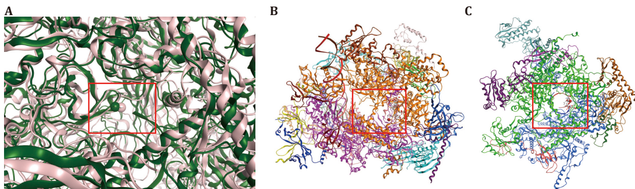
Fig. 1 Structural comparison and binding site prediction of ASFV and Sus scrofa RNA polymerases. A Structural superposition of ASFV RNAP (dark green; PDB: 8XX4) and Sus scrofa Pol II (pink; PDB: 7NVS). The red box indicates the conserved Mg^{2+} -binding site. B Predicted druggable pockets (red and gray spheres) near the Mg^{2+} site in Sus scrofa Pol II, identified using MOE. C Analogous predicted binding pockets in ASFV RNAP, used for virtual screening
