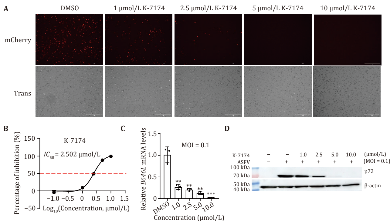
Fig. 4 Dose-dependent inhibition of ASFV by K-7174. A Fluorescence imaging of ASFV-infected PAMs treated with K-7174. B Dose-response curve of K-7174, with an IC_{50} value of 2.502 μmol/L. C Transcript levels of the late gene B646L (p72) measured by RT-qPCR. D Protein levels of p72 analyzed by Western blot. Data are presented as mean ± SD from three independent experiments. Statistical significance was determined using GraphPad Prism 8 (** P < 0.01 ; *** P < 0.001 )
