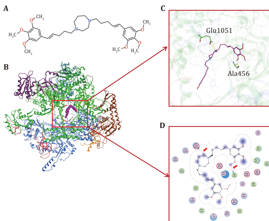
Fig. 5 Molecular docking analysis of K-7174 bound to ASFV RNAP. A Chemical structure of K-7174. B Overall binding pose of K-7174 within the catalytic pocket. C Detailed 3D view of key interactions; green: carbon, red: oxygen, blue: nitrogen; yellow dashed lines: hydrogen bonds. D 2D interaction diagram highlighting hydrogen-bond contacts
