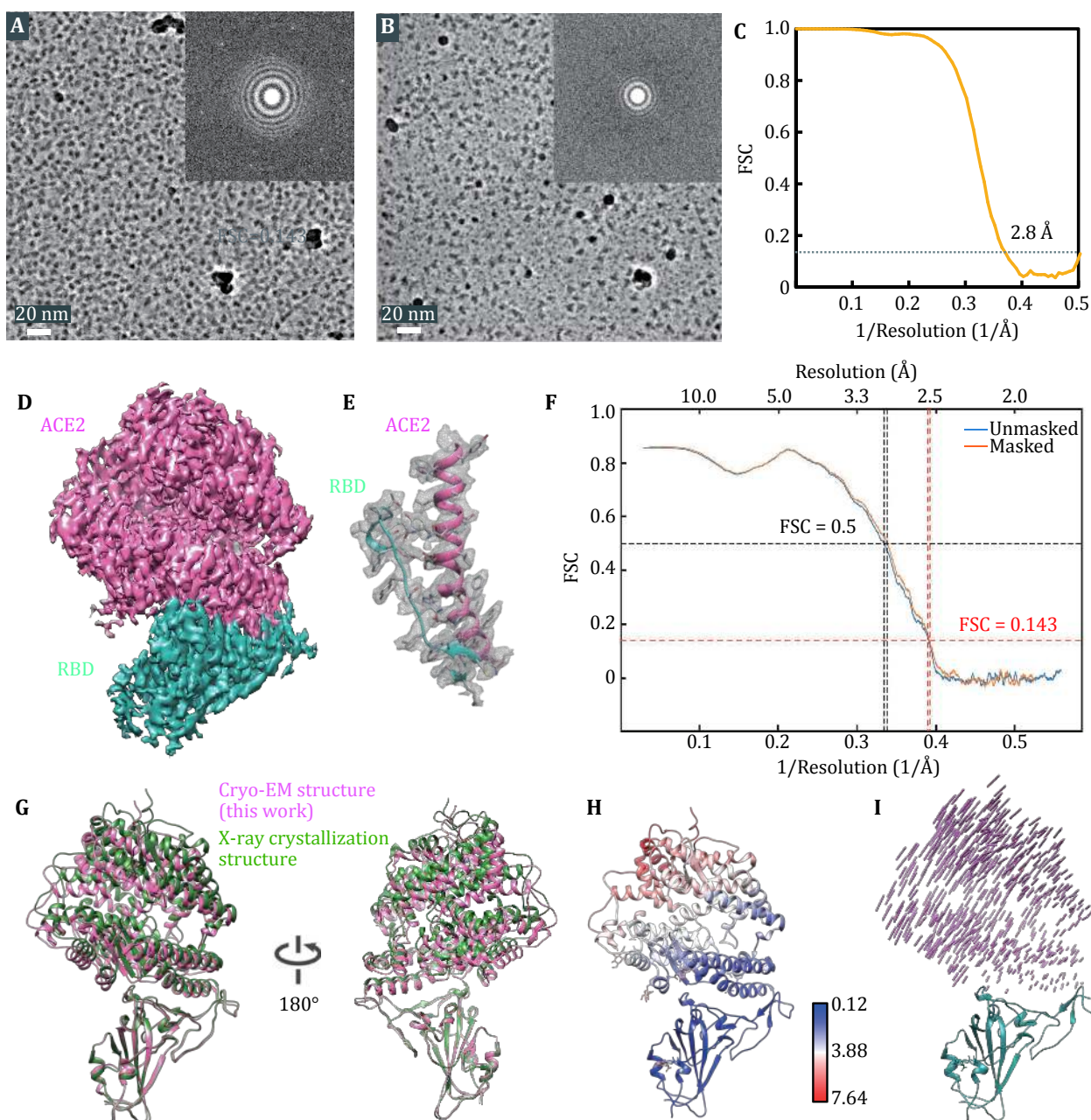
Fig. 5 Cryo-EM reconstruction of ACE2-RBD complex supported by RGO membrane. A A representative micrograph of RBD-ACE2 complex in the RGO supporting area. The inset was the corresponding FFT image, where six first-order diffraction spots of graphene were sharply displayed. B A representative micrograph of RBD-ACE2 complex in the RGO-broken area. C The FSC curve of ACE2-RBD complex reconstruction. The dotted gray line indicated FSC = 0.143, which was used for estimating the resolution. D The cryo-EM density of ACE2-RBD complex. The pink region was ACE2, while the cyan was RBD. E The ACE2-RBD interaction interface with their atomic models docked. F The ACE2-RBD model-map FSC curve. G Comparison between the cryo-EM structure solved in this work (colored in pink) with the reported X-ray crystal structure (PDB: 6M0J, in green). H RMSD (Å) between the cryo-EM structure and the X-ray crystal structure. I 3D vector map between the cryo-EM structure and the X-ray crystal structure, using RBD as the alignment reference. The vector lengths indicated the displacement scale across these two structures
